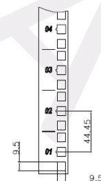
Upright detail
